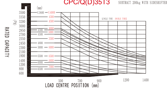
RATED CAPACITIES AND LOAD CENTERS GRAPH
