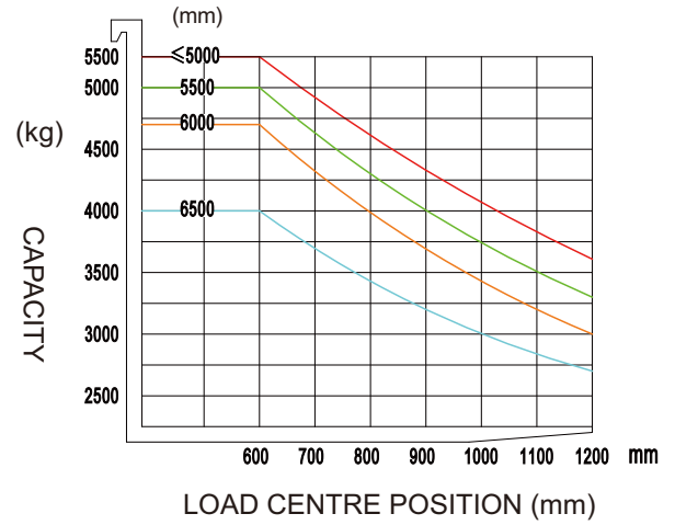
EFL553-HVD-6 RATED CAPACITIES AND LOAD CENTERS GRAPH
