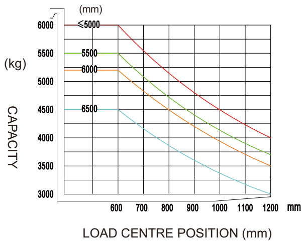
EFL603-HV-6 RATED CAPACITIES AND LOAD CENTERS GRAPH
