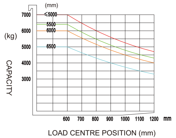
EFL703-HV-6 RATED CAPACITIES AND LOAD CENTERS GRAPH
