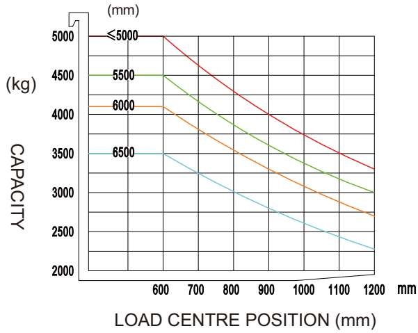
EFL503-HVD-6 RATED CAPACITIES AND LOAD CENTERS GRAPH
